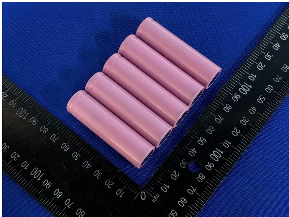
Figure 6 Side view-2 of cell for model IMR18650-800mAh
