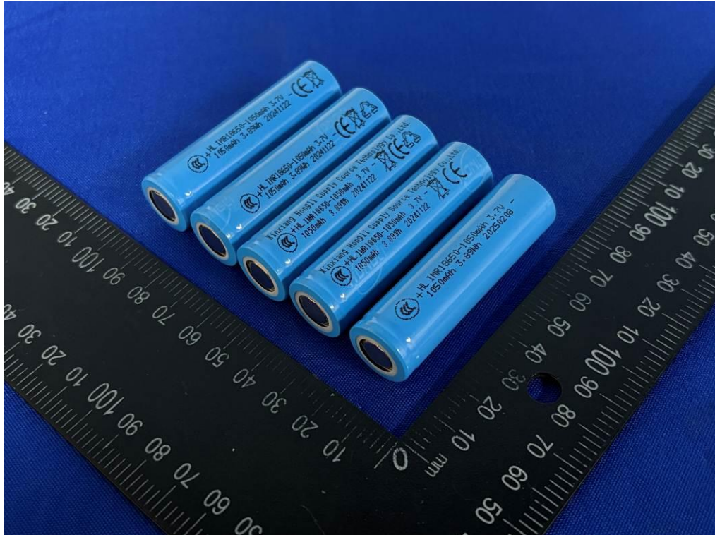
Figure 7 Side view-1 of cell for model IMR18650-1050mAh
