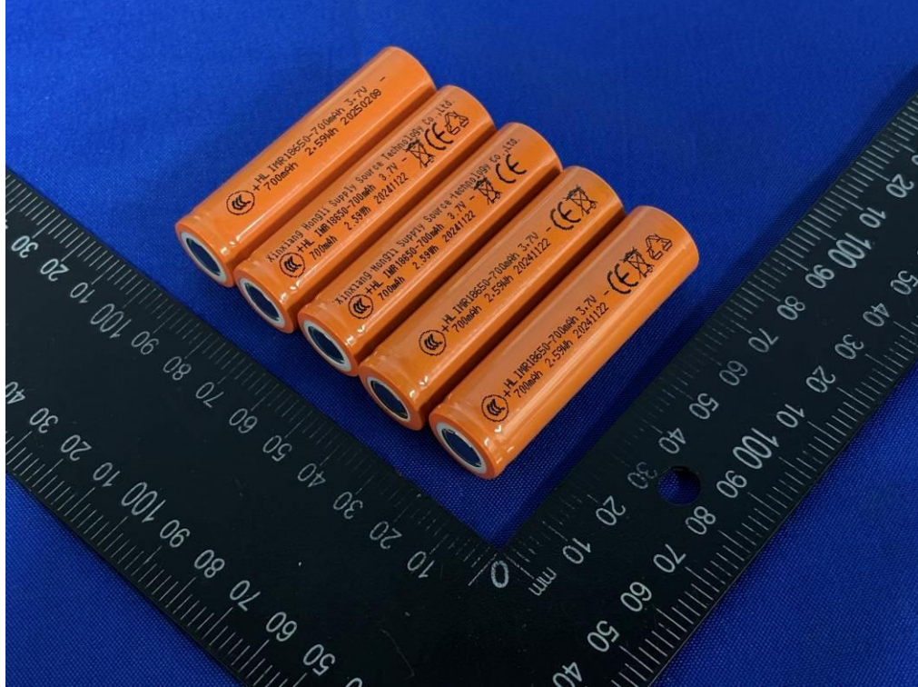
Figure 3 Side view-1 of cell for model IMR18650-700mAh
