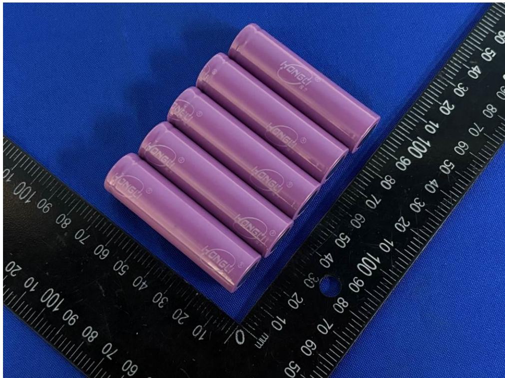
Figure 10 Side view-2 of cell for model IMR18650-1200mAh
